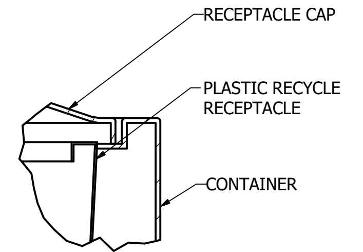
DETAIL B
