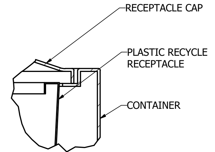
DETAIL B
